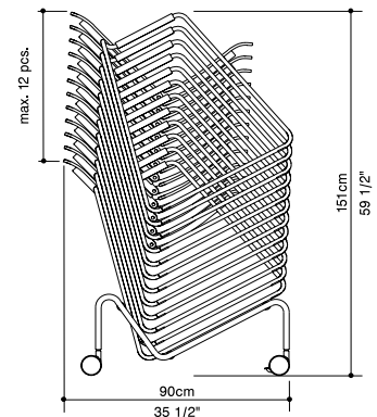
ST.HC with 12 SEATTABLES stacked as chairs
